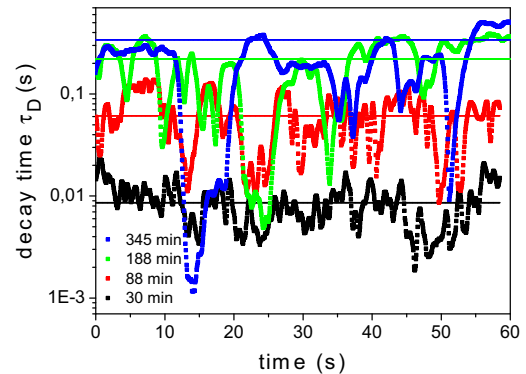
Fig. 5. Temporal dependence of the DWS decay time for a foam of 19% liquid fraction for several ages of the foam. In addition to an overall increase of the average decay time due to the coarsening of the foam, a marked change in the dynamics can be seen. At late age, the dynamics is dominated by intermittent burst of activity corresponding to large scale rearrangements of bubbles, which decrease in frequency as the foam coarsens.
