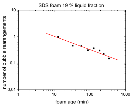
Fig. 7. The rearrangement frequency in a foam of 19% liquid fraction. The frequency scales with the foam age ^{-1/2} , as indicated by the solid line. The rearrangement frequency is given in s^{-1} .
