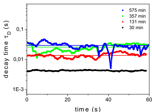
Fig. 6. Temporal dependence of the DWS decay time for a foam of 34% liquid fraction for several ages of the foam. In contrast to the relatively dry foam of Fig. 5, the dynamics is here not dominated by single events, but rather by random fluctuations. In addition, the time scale of the decay time is much faster, connected to the ballistic motion of bubbles between collisions.
