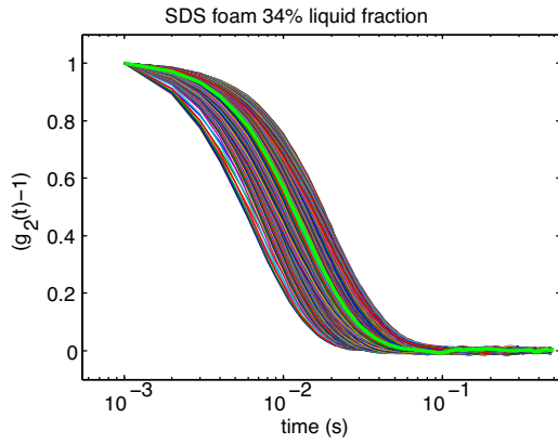
Fig. 3. Correlation function from multiple speckles obtained with a fast camera. The different curves correspond to different times in the foam on the scale of seconds showing large fluctuations in the temporal dynamics of the scatterers.
