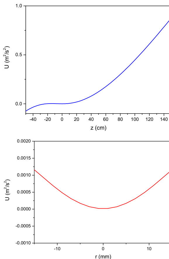
Fig. 1. Potential energy landscape in the vertical ( z ) and radial ( r ) directions. As can be seen, up to distances of a few mm in both r and z , the residual accelerations from these potentials are less than 0.001 g.
