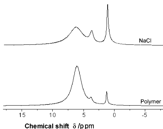
Figure 8. 1 H MAS NMR measurements of titania particles obtained by addition of salt and by polymer.
