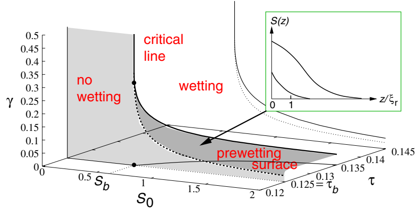
Figure 3. Wetting phase diagram for the planar geometry. In the parameter region (S_0, \gamma) of the light-grey shaded plane a wetting transition does not occur. The prewetting surface (dark-grey shaded surface) ends in a critical line. The additional full and dotted curves indicate the respective projection of the prewetting surface on the (S_0, \tau) plane or the (S_0, \gamma) plane at \tau = 0.145 . For a detailed explanation see the text.
