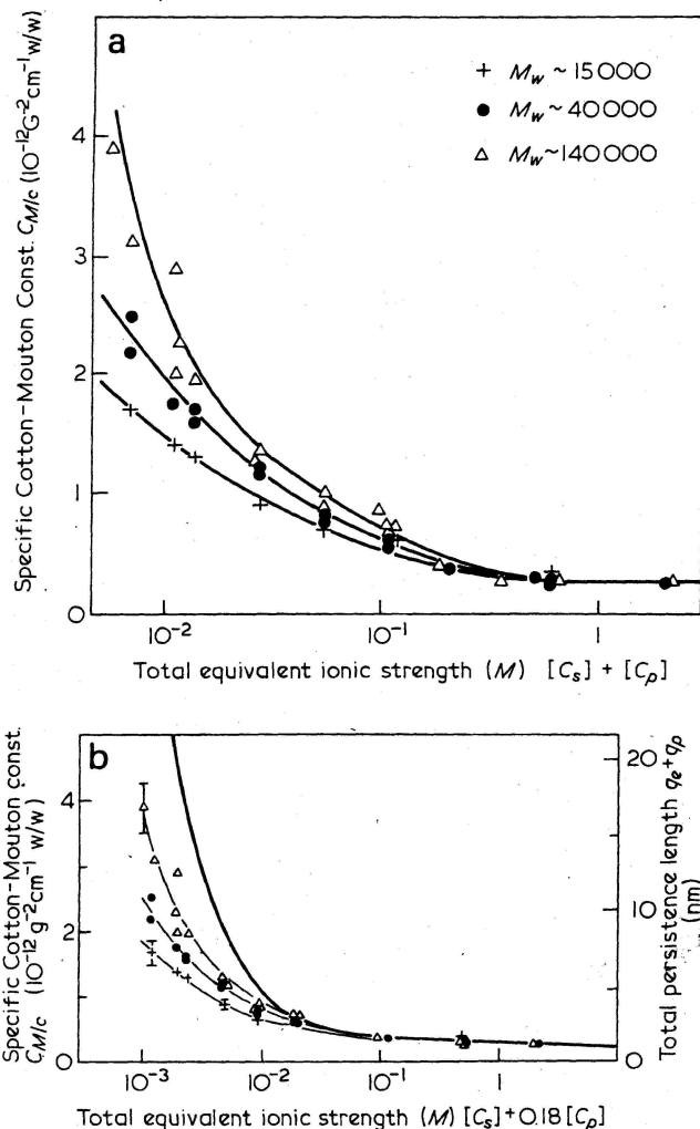
Figure 1 Specific Cotton-Mouton constant of PSS Na + as a function of the ionic strength: (a) calculated from the total monomolar concentration in polyion and salt; (b) calculated with only the uncondensed counterions. The heavy line has been calculated assuming a change in electrostatic persistence length according to eqs. 16 and 17
