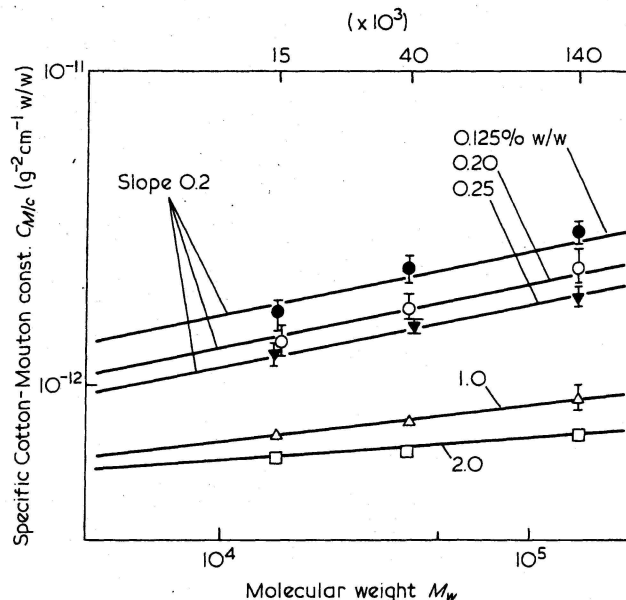
Figure 2 Log-log plot of the molecular weight dependence of the specific Cotton-Mouton constant of PSS \text{Na}^+ in the low concentration range in the absence of added salt
